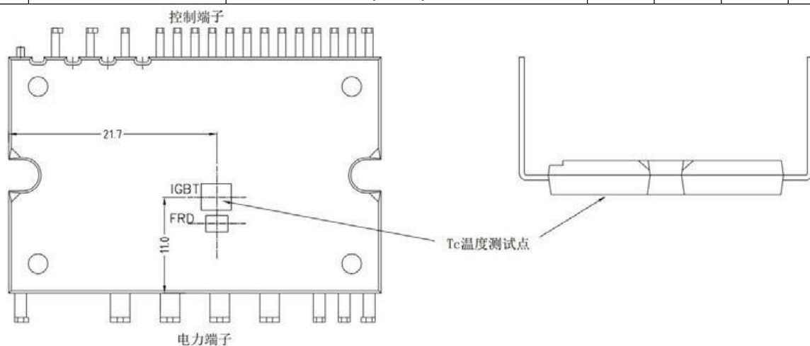
Fig.1 Tc MEASUREMENT POINT
