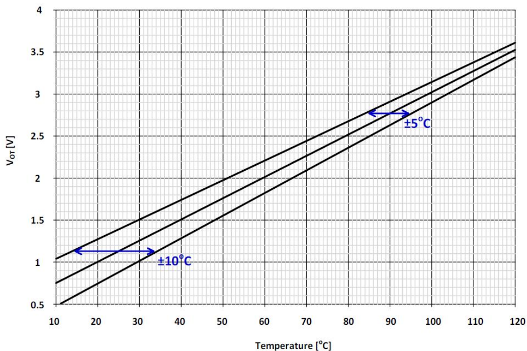
Fig.3 Temperature Profile of VOT(Typical)
