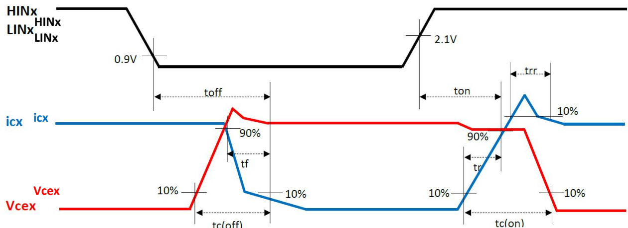
Fig.2 Switching times definition
